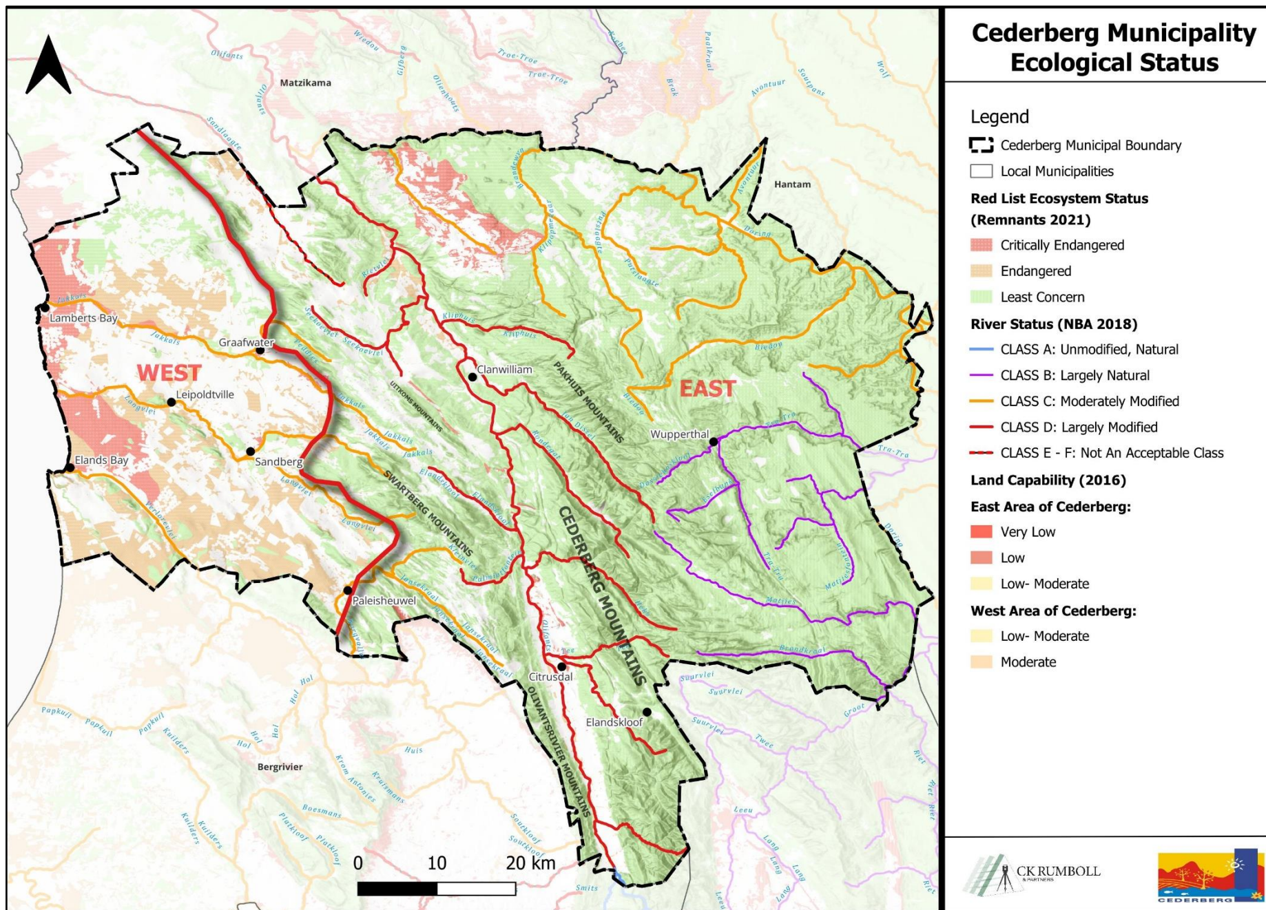
Map 8: Ecological Status of Cederberg
