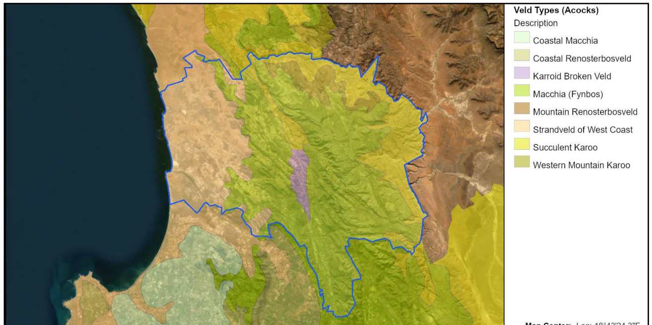
Map 7: Cederberg Vegetation Types
