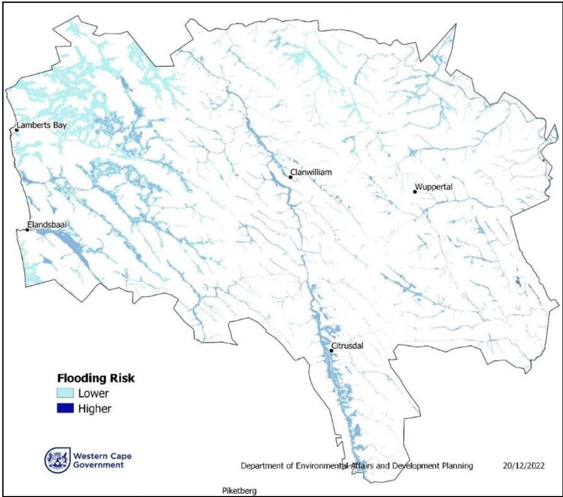
Map 17: Flood Risk in Cederberg, as a composite of likely flood area, flood likelihood and vulnerability (DEA&DP, 2022)
